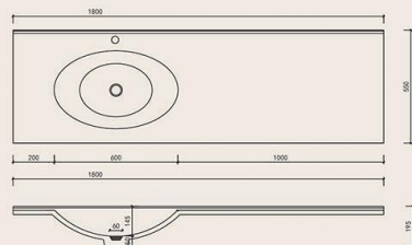
MT003 1800*550*195mm
