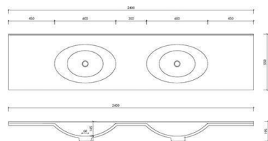
MT002 2400*550*195mm
