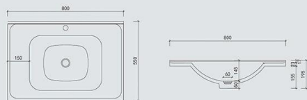
MT008 800*550*195mm
