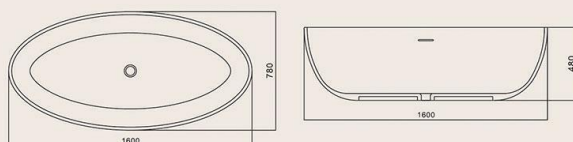
MY007 1600*780*480mm
