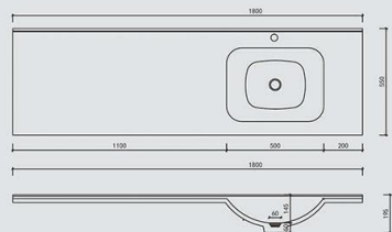
MT004 1590*745*595mm
