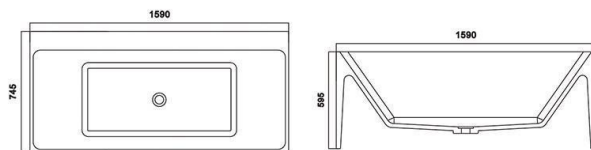
MY004 1590*745*595mm
