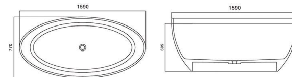
MY008 1590*770*605mm
