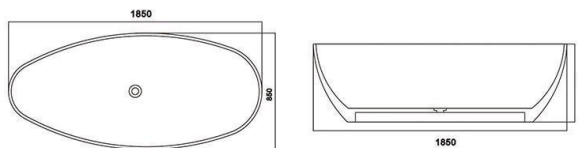
MY003 1850*850*570mm
