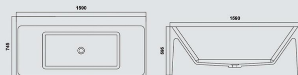
MY004 1590*745*595mm
