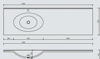
MT003 1800*550*195mm
