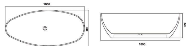
MY003 1850*850*570mm
